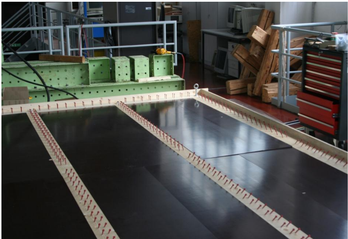
Assembled timber frame of the slab with formwork
