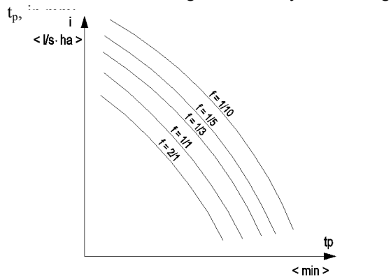
Fig.4 Diagram of rain calculation intensity in sewerage
