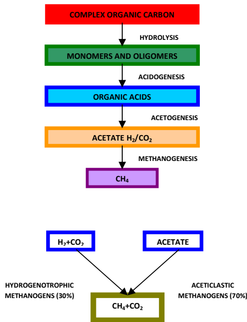
Fig.2. Anaerobic digestion biochemical conversion pathways
