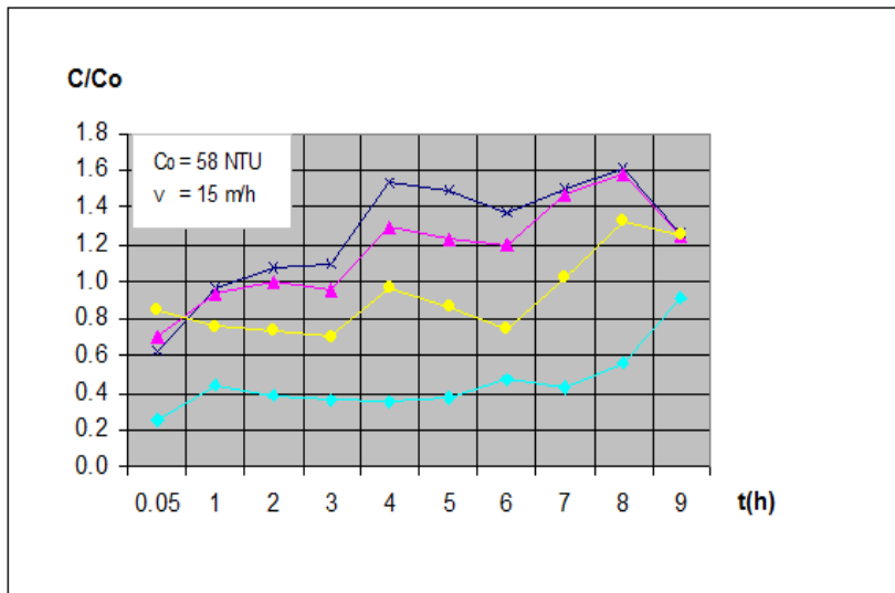
Figure 6. Qualitative changes over the filtration cycles for v = 15 m/h
