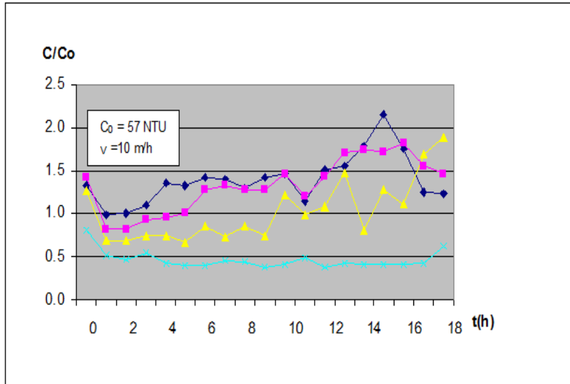
Figure 5. Qualitative changes over the filtration cycles for v = 10 m/h
