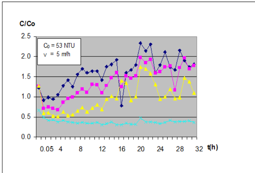
Figure 4. Qualitative changes over the filtration cycles for v = 5 m/h
