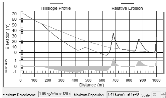
Figure 5. Soil loss graph for 5 min torrential rain duration and land use overgrazing
