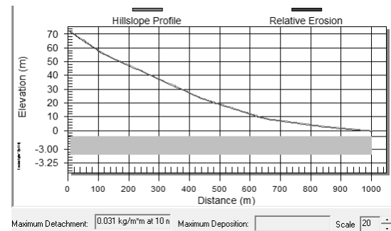
Figure 10. Soil loss graph for 60 min torrential rain duration and land use grass
