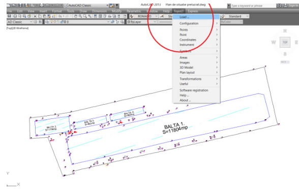
Figure 7. TopoLT Software
