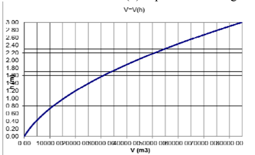
Figure 4 The construction curve Q = Q(h)
