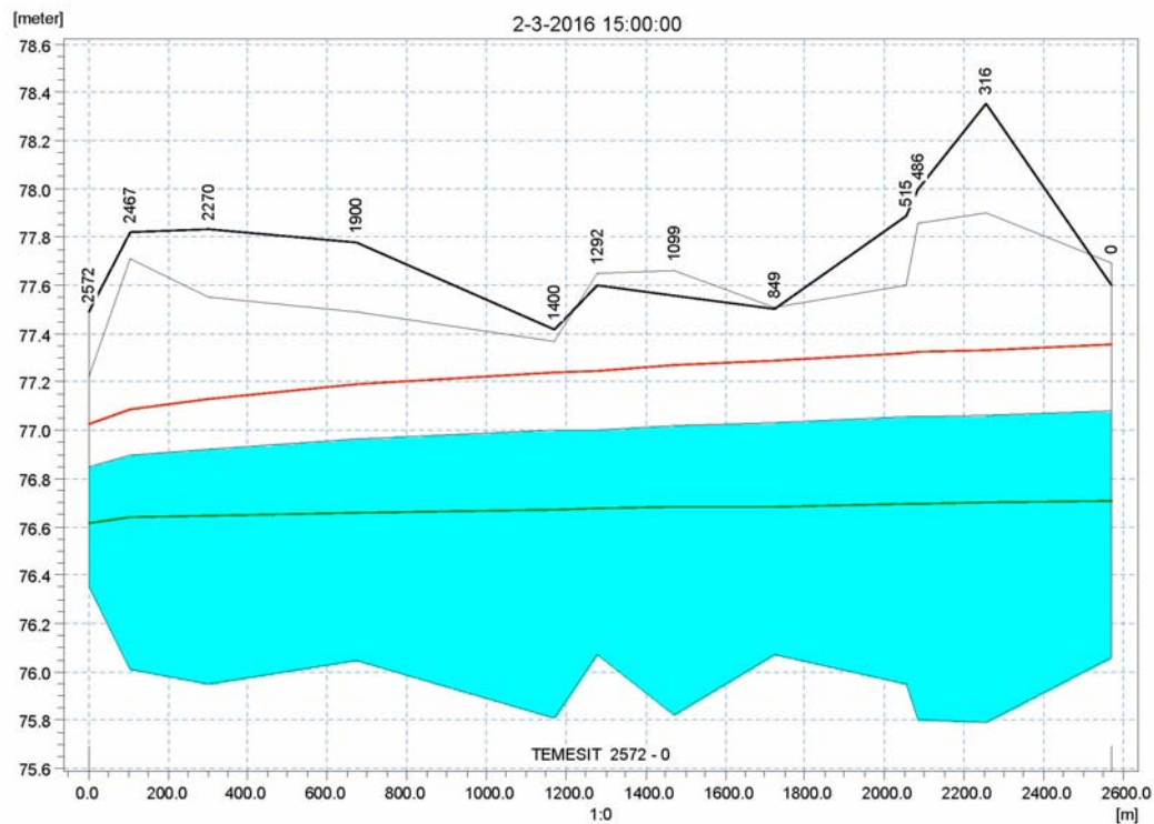
Figure 8 Longitudinal profile
