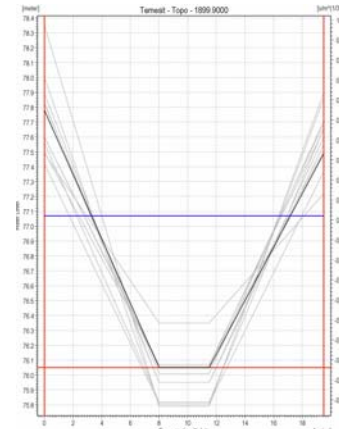
Figure 6 Cross sections
