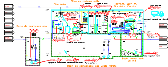
Figure 3. Wastewater pre-treatment station – technological process
