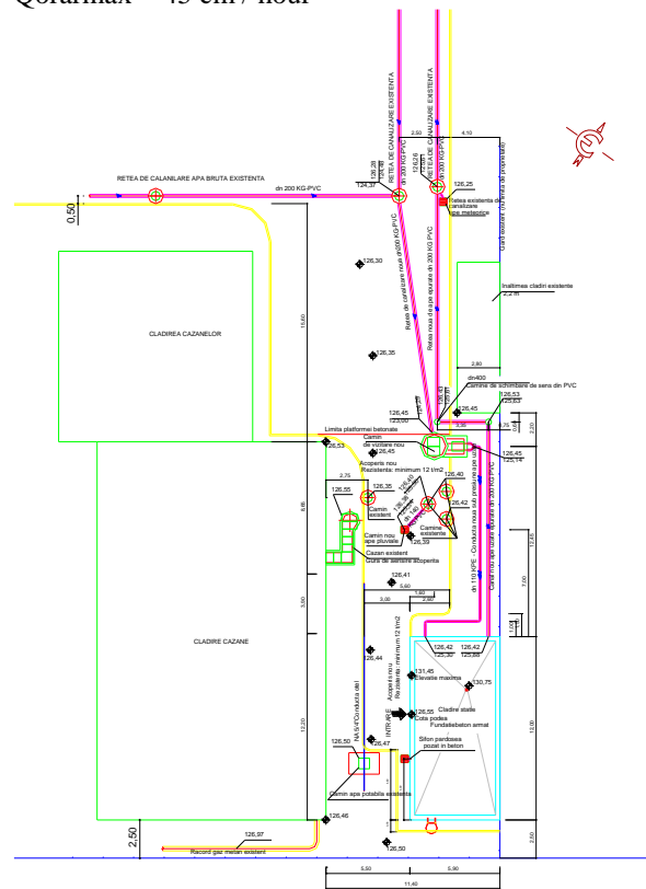
Figure 2. Wastewater pre-treatment station-hydraulics
