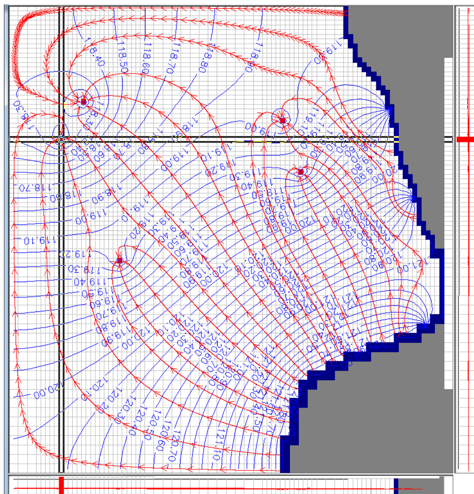
Figure 5. Contour lines
